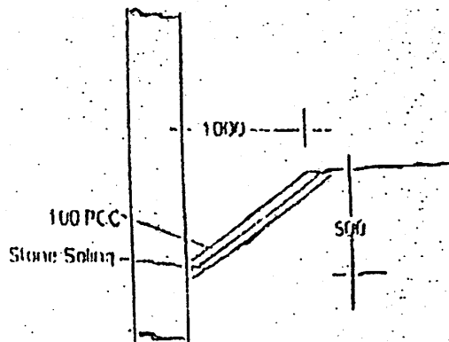
SAUCER DRAIN
