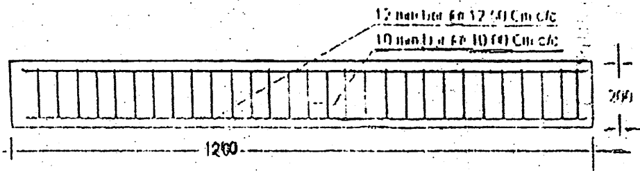
COVER SLAB
